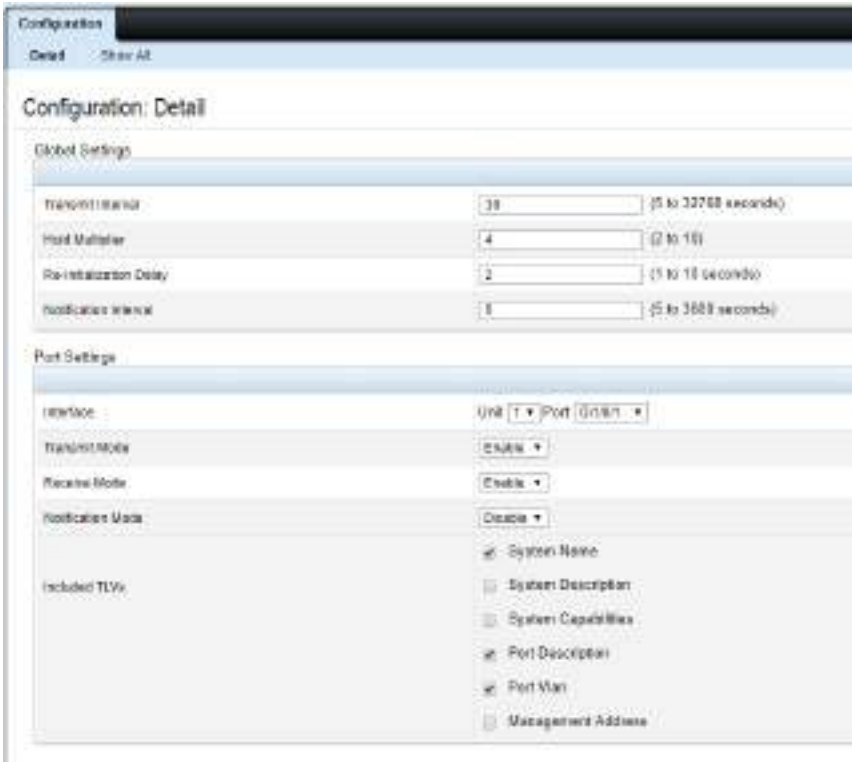
Figure 22-6. LLDP Configuration
