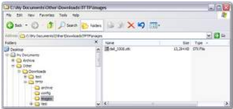
Figure 13-9. Image Path
