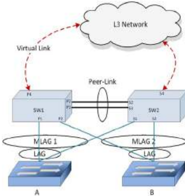
Figure 28-10. MLAG Components
