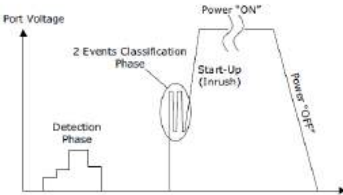
Figure 2-1. PD Detection
