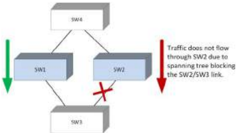
Figure 28-8. STP Blocking
