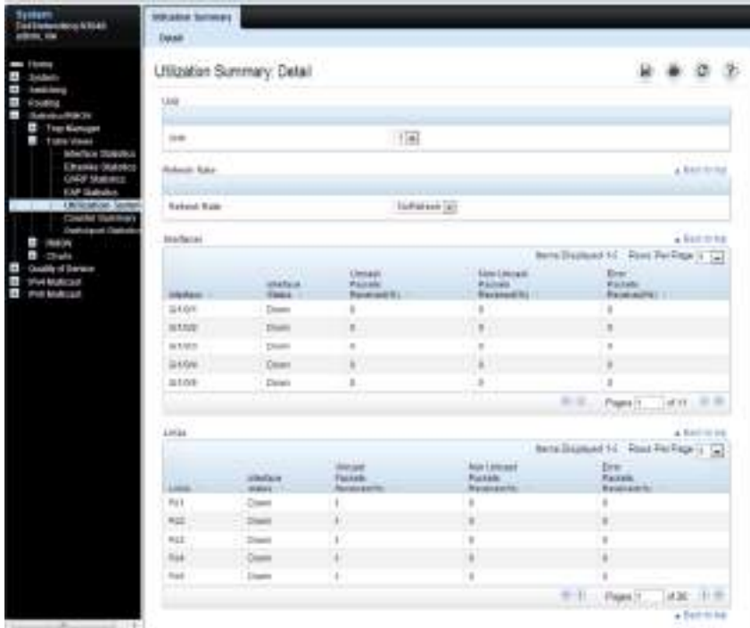
Figure 15-10. Utilization Summary
