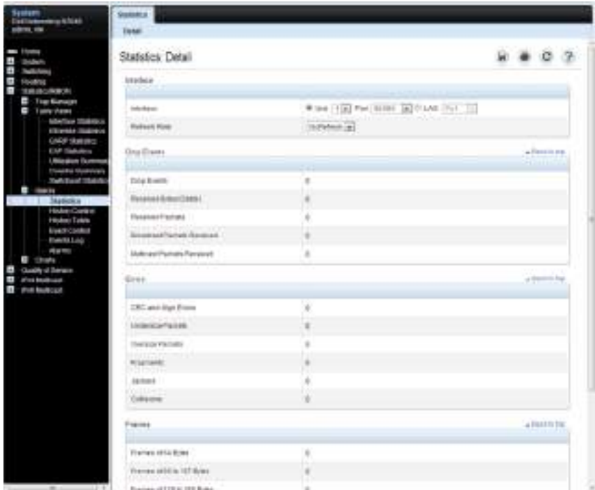
Figure 15-13. RMON Statistics
