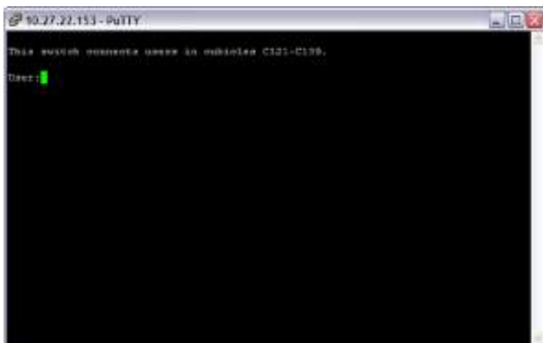
Figure 11-25. Verify MOTD
