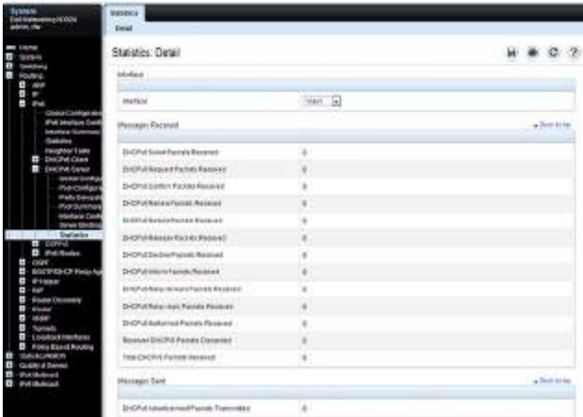
Figure 42-11. DHCPv6 Statistics
