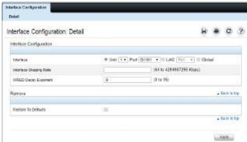
Figure 44-3. Interface Configuration
