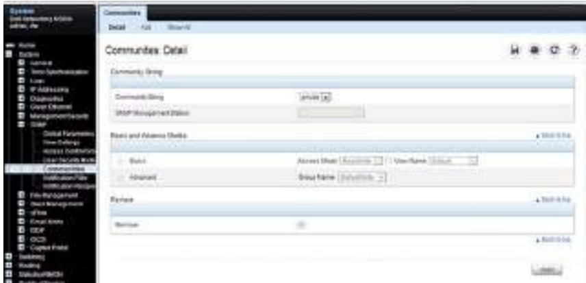
Figure 12-9. SNMP Communities
