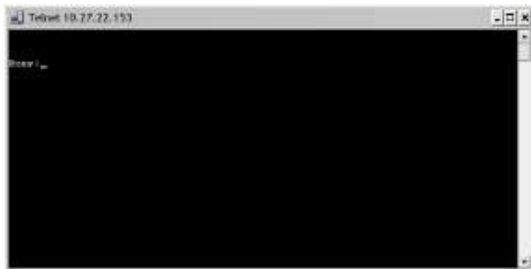
Figure 11-4. Telnet Session
