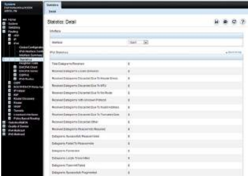
Figure 41-4. IPv6 Statistics
