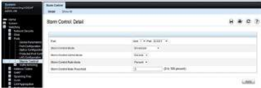
Figure 23-2. Storm Control
