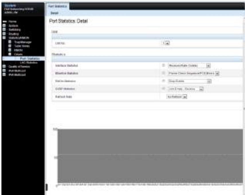
Figure 15-22. Ports Statistics
